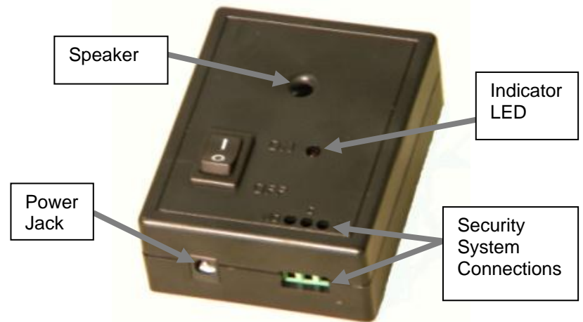
Figure 9 Receiver
